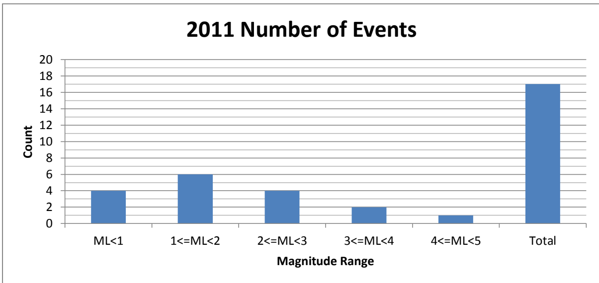
Figure 2: 2011 Earthquake Magnitude Frequencies.
