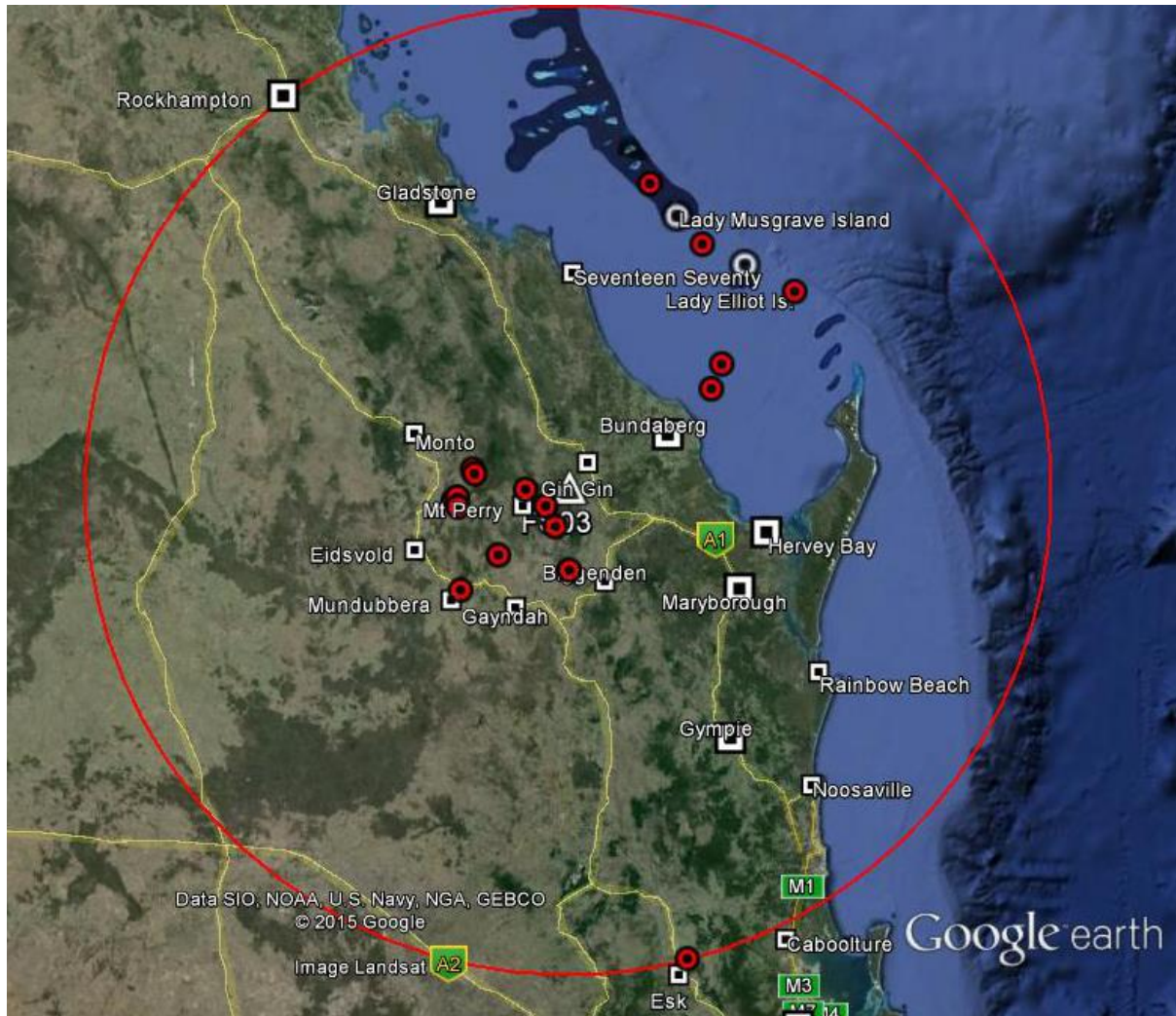
Figure 3: 2011 Earthquake Locations.
